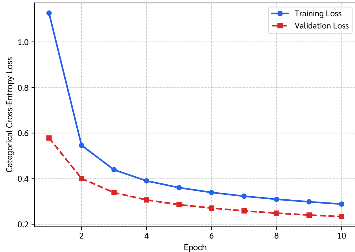
Training & Validation Loss over Epochs
