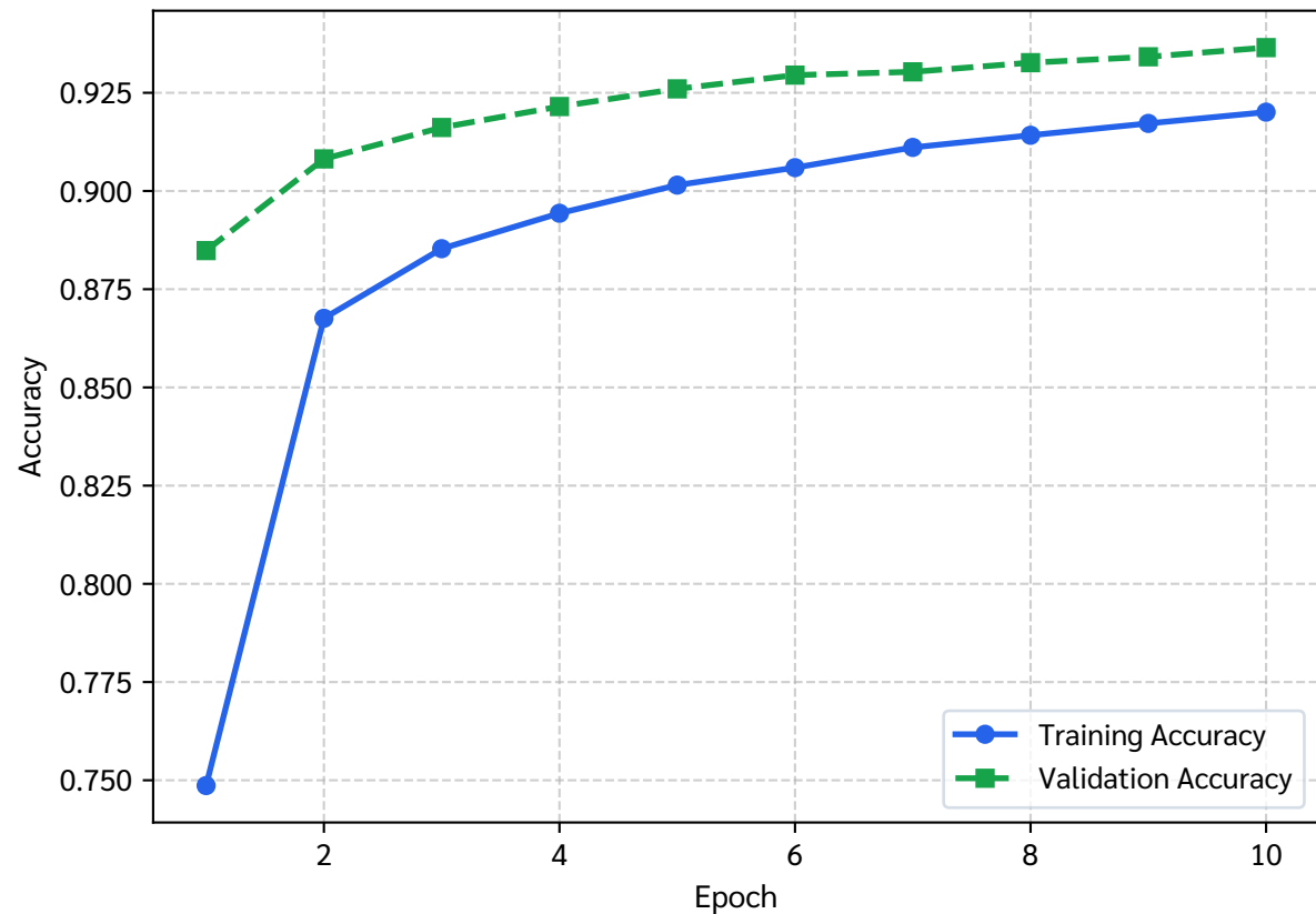
Training & Validation Accuracy over Epochs
